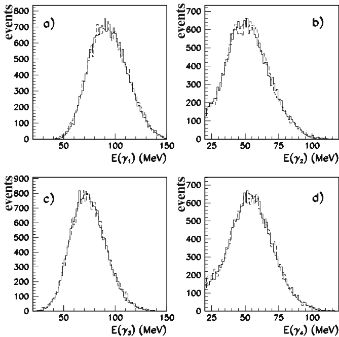
Fig. 5. Spectra of K_{\pi 3} : a energy of E_{\gamma 1} ; b energy of E_{\gamma 2} ; c energy of E_{\gamma 3} ; d energy of E_{\gamma 4} . The solid lines are the experimental data and the dashed lines are the MC predictions
