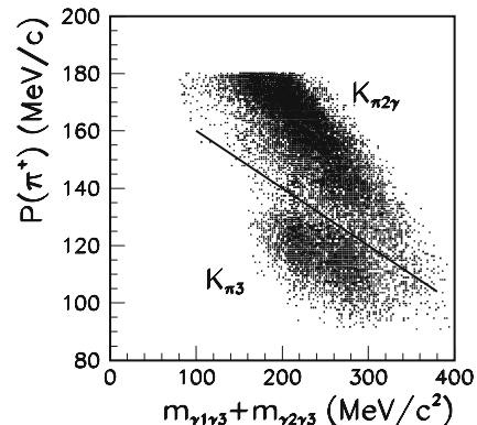
Fig. 3. Scatterplot of the \pi^+ momentum versus the sum of “invariant masses” comprised of \gamma_1, \gamma_3 and of \gamma_2, \gamma_3 . The shown line is a cut condition to remove the K_{\pi 3}
