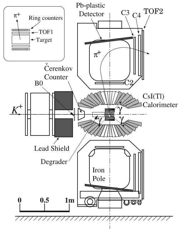
Fig. 1. The layout of the detector for E470 experiment
