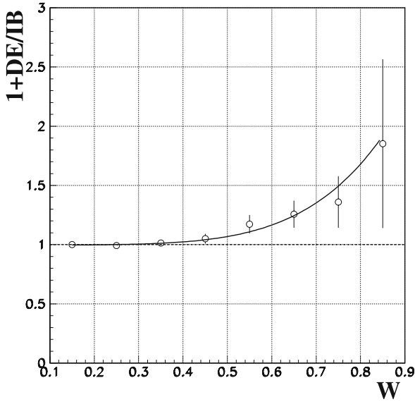
Fig. 7. W spectrum of the observed K^+ \rightarrow \pi^+\pi^0\gamma events normalized to the IB component obtained from the Monte Carlo simulation. The solid curve shows the best fit of the W spectrum to a sum of the IB and DE components
