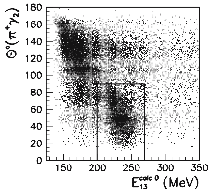
Fig. 2. Scatterplot of \theta_{\pi^+ \gamma_2} vs E_{13}^{\text{calc0}} . Here, \theta_{\pi^+ \gamma_2} is the opening angle between \pi^+ and \gamma_2 , and E_{13}^{\text{calc0}} is the parameter E_{\pi^0(\gamma_i \gamma_j)}^{\text{calc0}} with i = 1, j = 3 . The region enclosed in the rectangular box is a region of incorrect photons pairing
