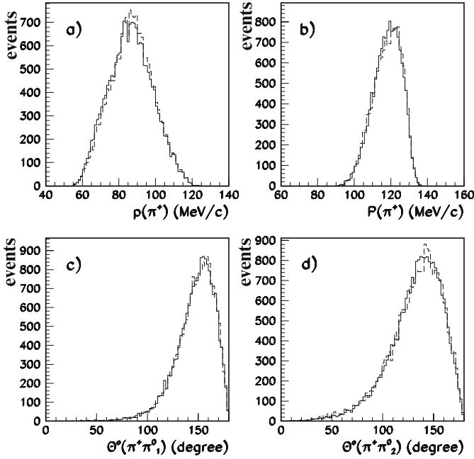
Fig. 4. K_{\pi 3} spectra: a \pi^+ momentum before correction for energy losses in the target; b \pi^+ momentum after correction for energy losses in the target. c opening angle between \pi^+ and \pi_1^0 ; d opening angle between \pi^+ and \pi_2^0 . The solid lines are the experimental data and the dashed lines are the MC predictions
