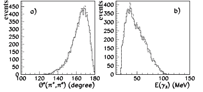
Fig. 6. Spectra of K^+ \rightarrow \pi^+ \pi^0 \gamma with an additional cut of W < 0.5 . a opening angle between the \pi^+ and the \pi^0 ; b energy of \gamma_3 . The solid lines are the experimental data and the dashed lines are the IB component from the Monte Carlo predictions
